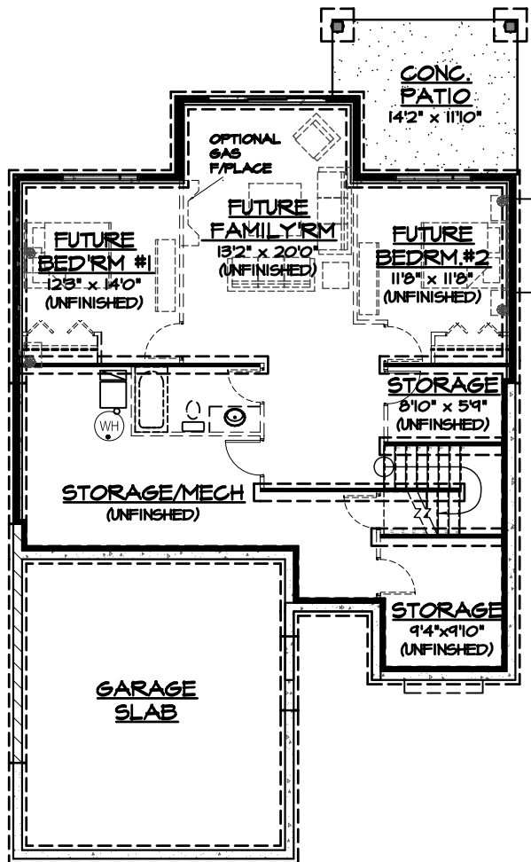
LOWER FLR PLAN 796 SQ/FT. SHOWN FUTURE (EXCLUDING STAIR)
