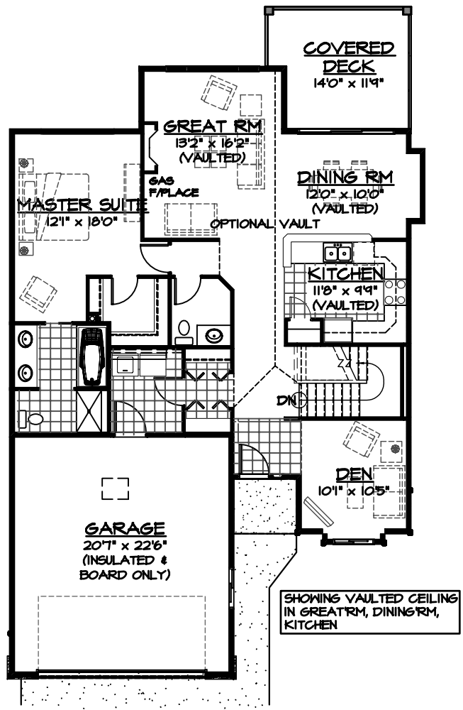
MAIN FLR PLAN 1364 SQ/FT.
