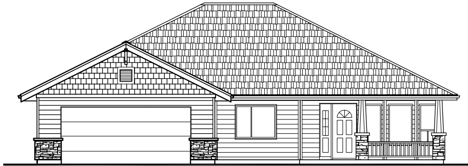
STREET ELEVATION
