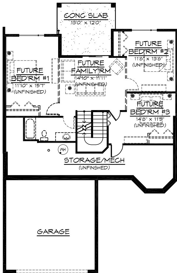
LOWER FLR PLAN 855 SQ/FT. SHOWN FUTURE (EXCLUDING STAIR)
