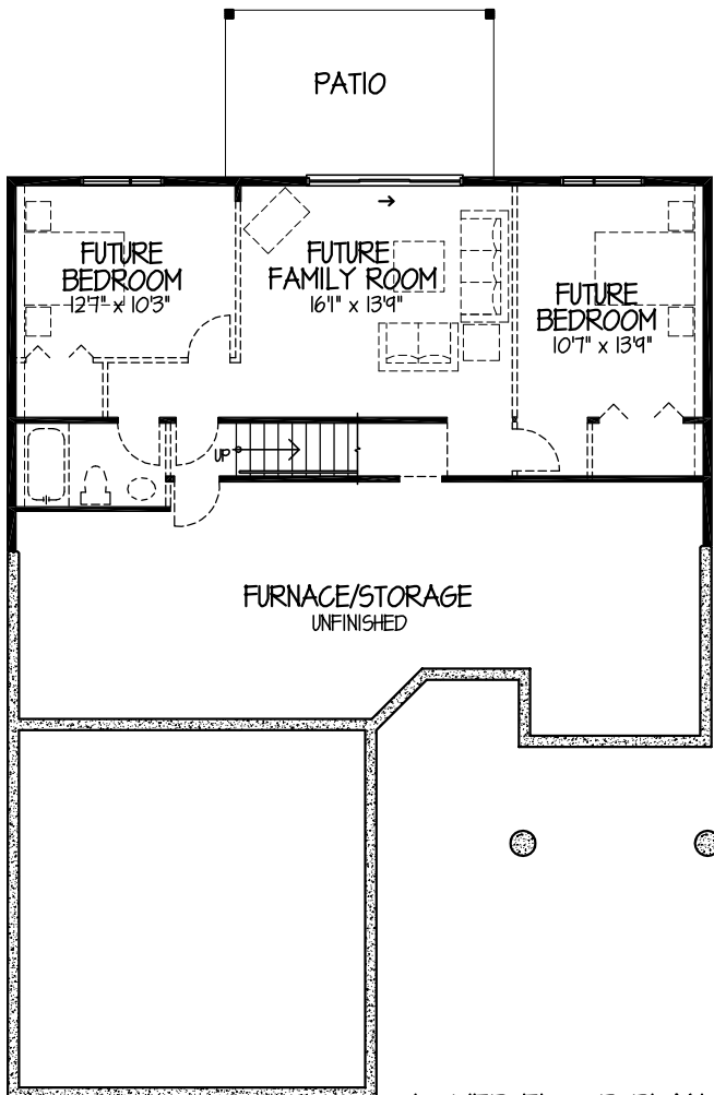
LOWER FLOOR PLAN 743 sq.ft. SHOWN FUTURE
