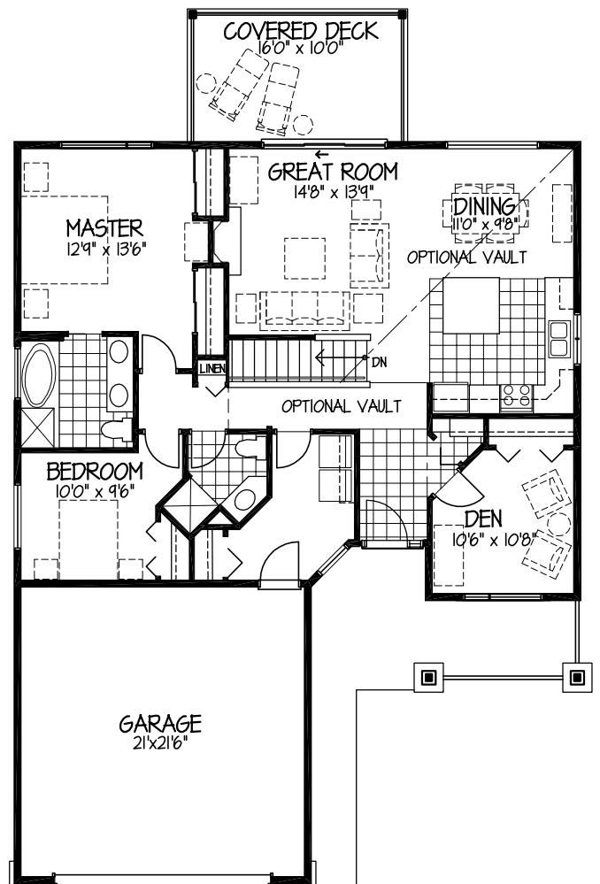
MAIN FLOOR PLAN 1377 sq.ft.
