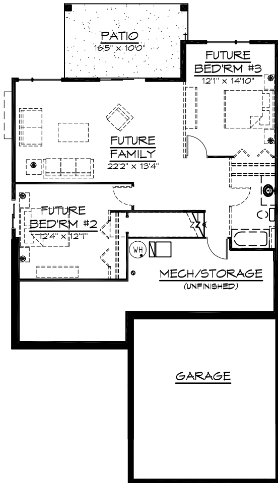
LOWER FLR PLAN 884 SQ/FT. SHOWN FUTURE (EXCLUDING STAIR)
